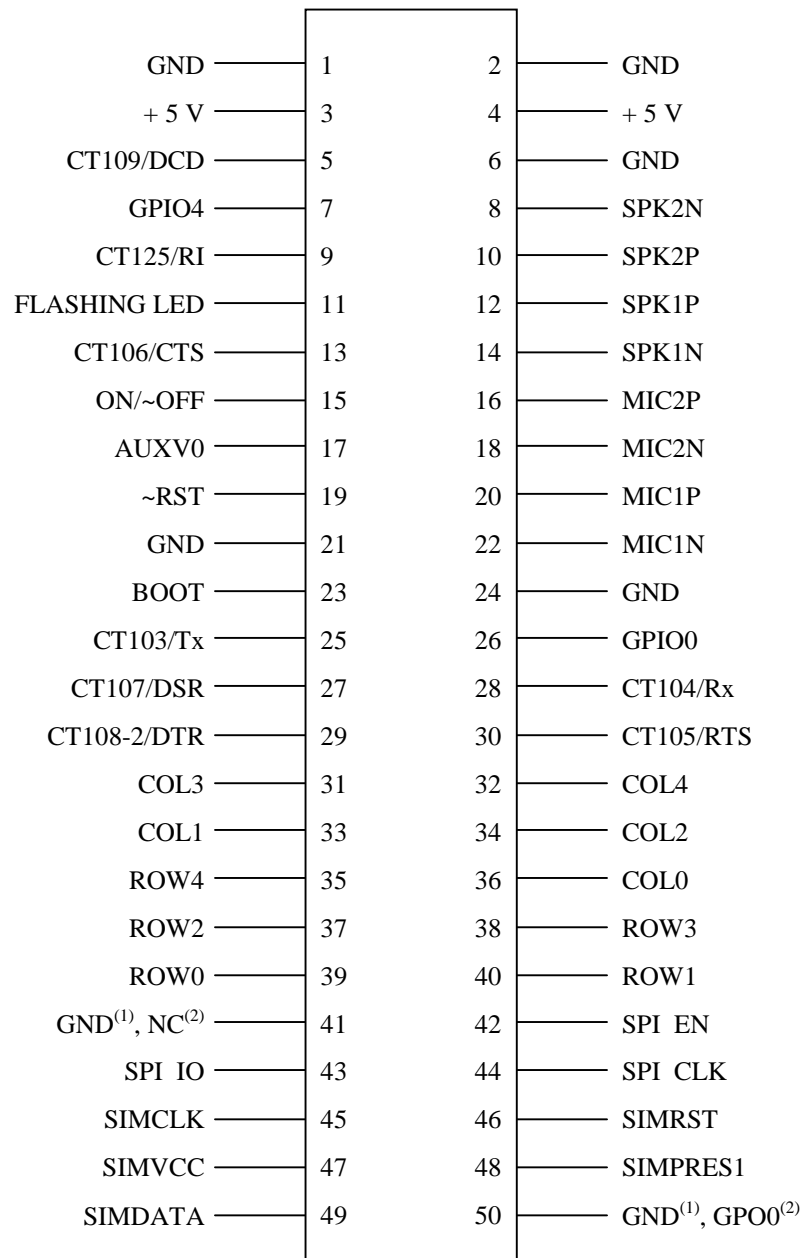
figure 3 : 50-pin connector
